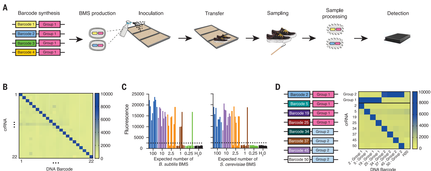
Fig. 1. BMS can be specifically and sensitively detected. (A) Schematic of the BMS application and detection pipeline. (B) Heatmap of endpoint fluorescence values from in vitro SHERLOCK reactions of all combinations of 22 barcodes and 22 crRNAs assessing specificity of each barcode-crRNA pair. (C) Detection limit of B. subtilis and S. cerevisiae BMS by SHERLOCK (each of the eight biological replicates for each spore concentration are shown). Spore numbers are calculated on a per-reaction basis. (D) Heatmap of endpoint fluorescence values from in vitro SHERLOCK reactions testing the specificity of four barcodes for group 1 crRNA and four barcodes for group 2 crRNA as detected by either specific or group crRNA.
