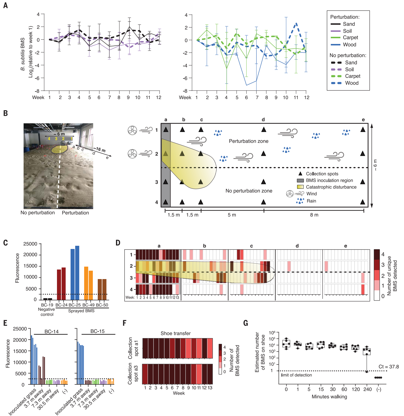
Fig. 2. Persistence, transferability, and maintenance of BMS. (A) BMS persisted on sand, soil, carpet, and wood over 3 months on ~1-m 2 test surfaces in incubators. The y-axis shows the B. subtilis BMS number relative to week 1 levels. Bars represent standard deviations. Perturbations were simulated wind, rain, vacuuming, or sweeping. (B) Photograph and schematic of a large-scale (~100-m 2 ) sandpit. B. subtilis BC-24 and BC-25 BMS and S. cerevisiae BC-49 and BC-50 BMS were inoculated in the shaded gray region in the diagram. The yellow shadow represents the area over which the top 5 cm of sand from a 1.5-m 2 area of the inoculation region was redistributed after a large fan fell over. (C) SHERLOCK signal from the four BMS from the inoculated region “a” in the large-scale experiment. Dashed line is the threshold for positive calls. BC-19 is the negative control. (D) BMS persist at
