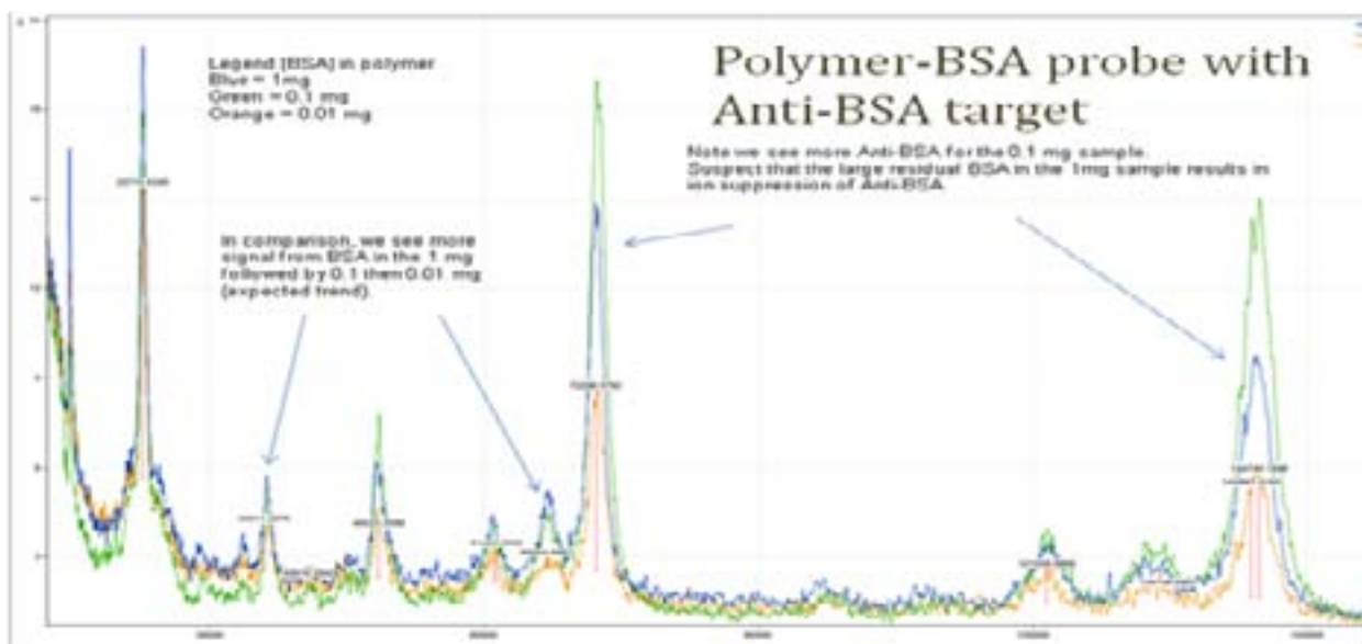
Demonstration of clear target recognition (anti-BSA) with very little probe contamination (BSA).
